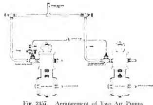
Fig. 2457. Arrangement of Two Air Pumps with One Complete Air Pump Governor and Steam Portion of Pump Governor.
